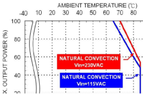
Derating Curve vs. Ambient Temperature TAC15USxxB xx=24/28/36/48/53 Connector Option : (□: JST)
