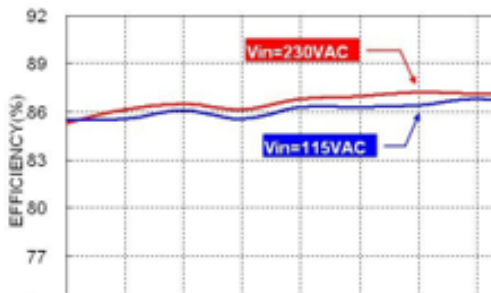
43TAC15US12B Efficiency vs. Output Load
