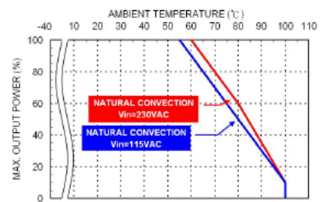
Derating Curve vs. Ambient Temperature TAC15USxxB xx=3P3/05/7P5/09/12/15/18 Connector Option : (-M / -T / -D)
