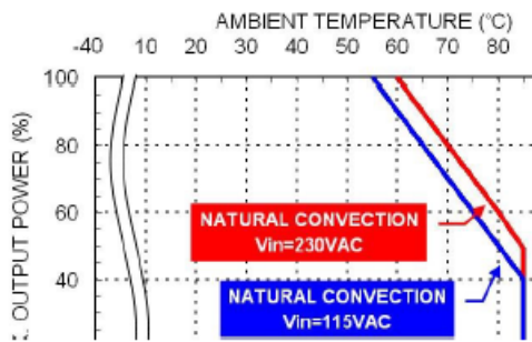
Derating Curve vs. Ambient Temperature TAC15USxxB xx=3P3/05/7P5/09/12/15/18 Connector Option : (□: JST)
