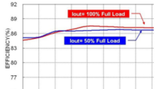
43TAC15US12B Efficiency vs. Input Voltage
