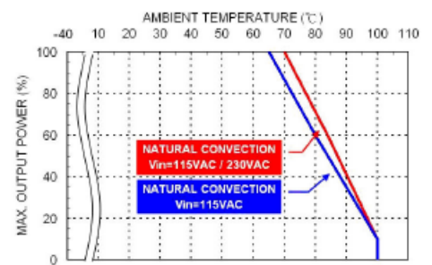
Derating Curve vs. Ambient Temperature TAC15USxxB xx=24/28/36/48/53 Connector Option : (-M / -T / -D)
